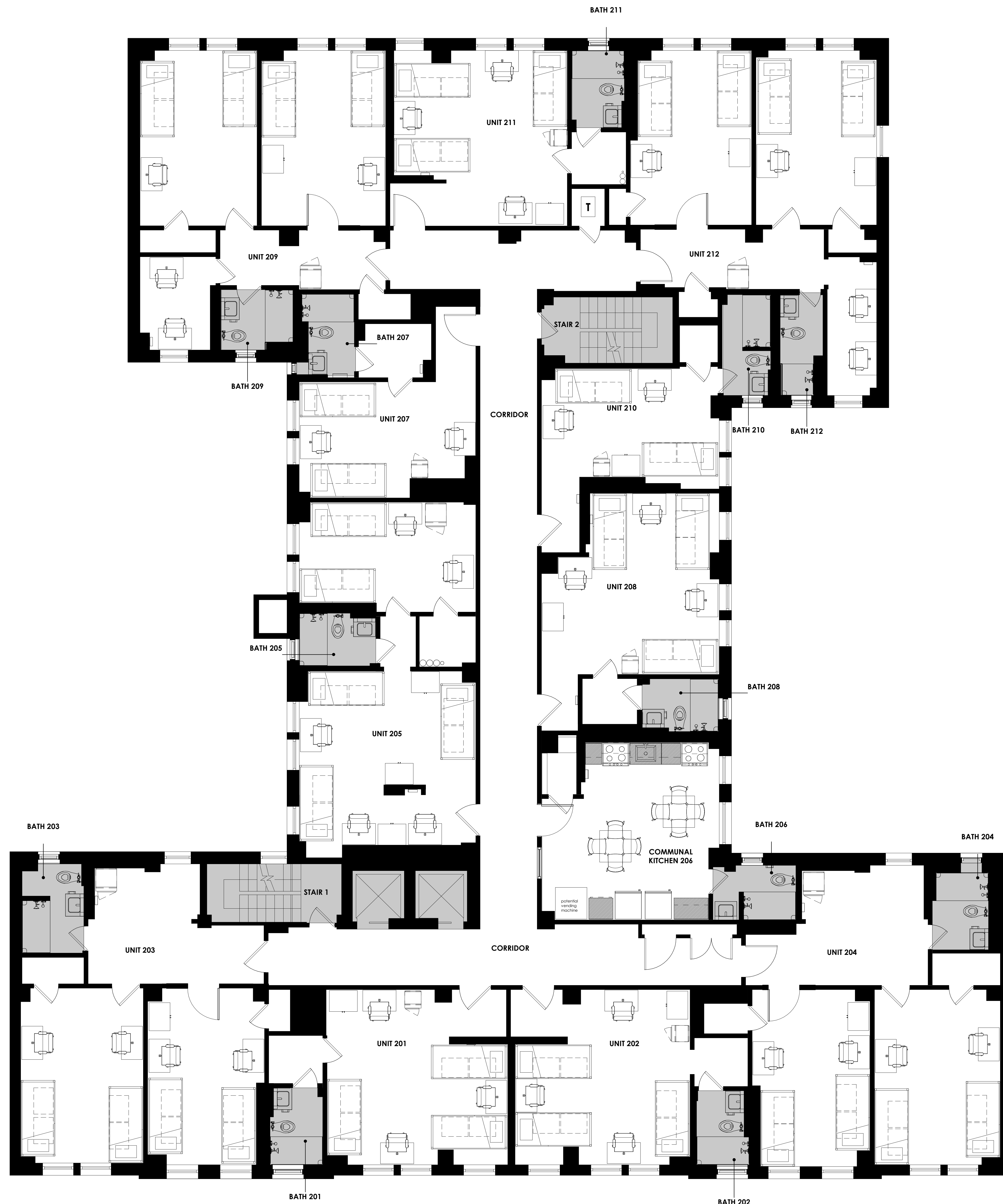
① SECOND AND SIXTH FLOOR COMMUNAL KITCHENS Scale: 1/4" = 1'-0"
