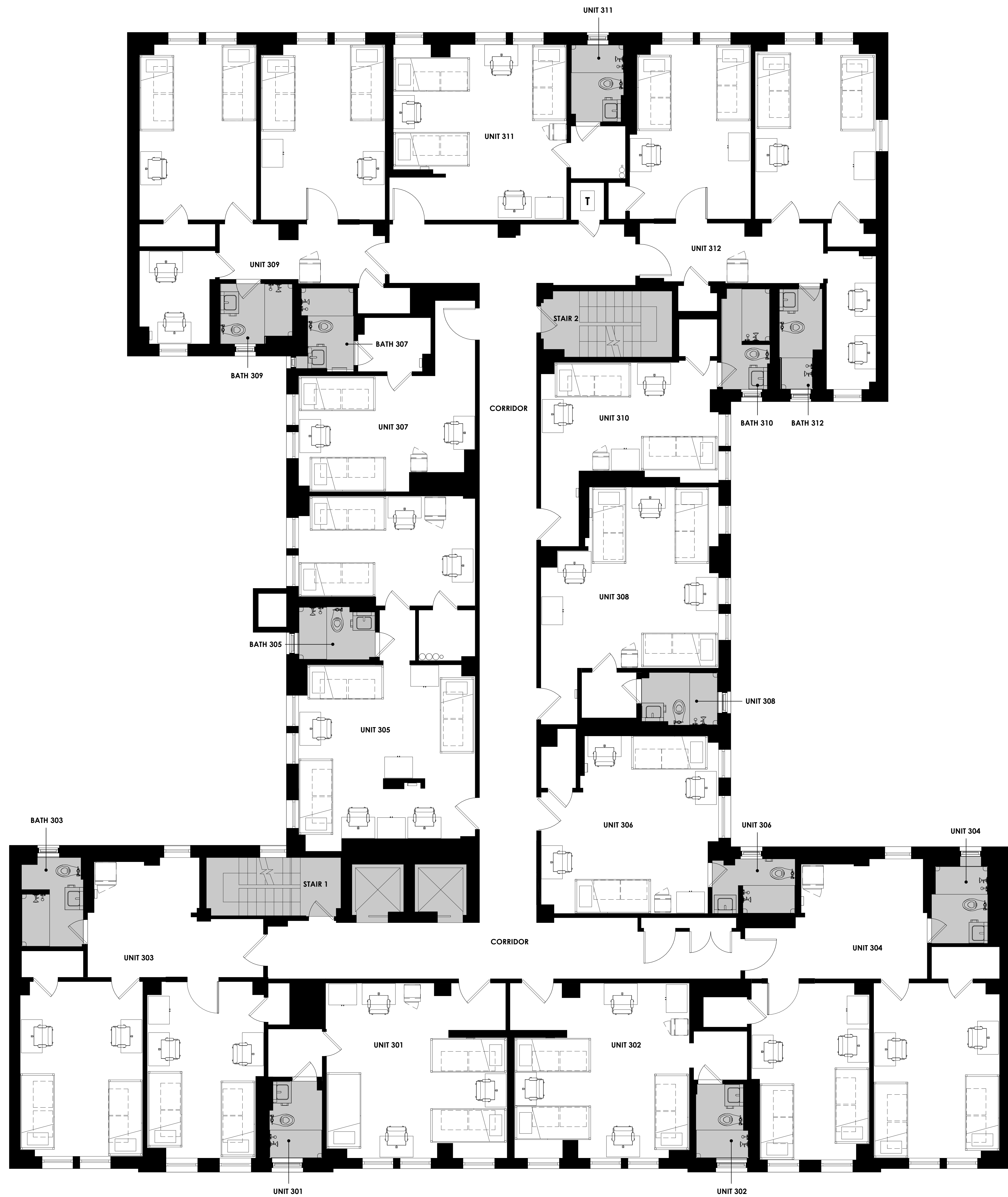
① TYPICAL NON-KITCHEN FLOORS Scale: 1/4" = 1'-0"
